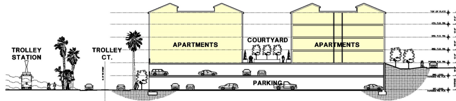
EAST PARCEL CROSS SECTION "B-B"
