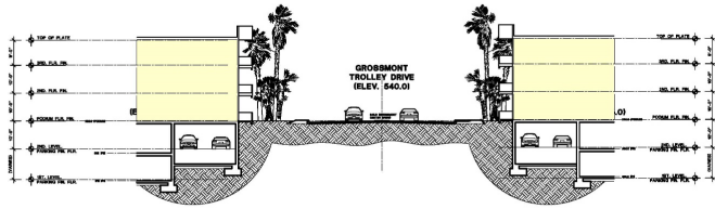
EAST AND WEST PARCEL CROSS SECTION "E-E"
